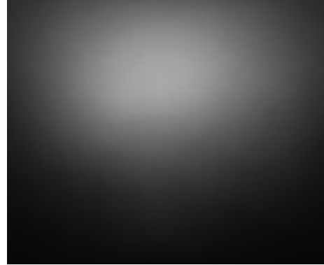
training set
