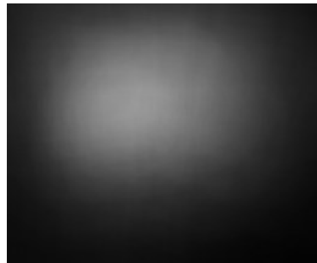
test set
